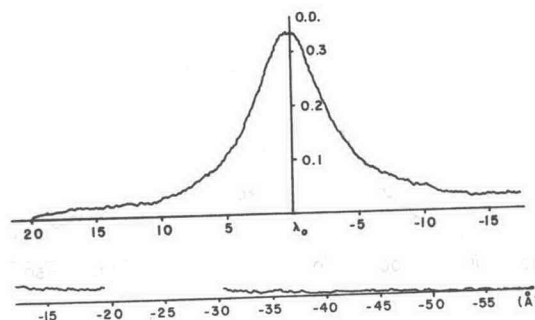
FIG. 5. Line shape of Ca 4227 in He. P = 2563\text{ psi} , T = 638^\circ\text{C} , \text{rd} = 50.7 .
