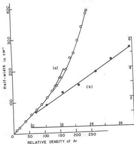
FIG. 4. Half-width of Ca 4227 in Ar. Curve (a): For high rd at 637^\circ\text{C} . Use the ordinate at the left and the abscissa at the bottom, where open circles are rd values computed with Beattie-Bridgeman equation; open triangles, those according to Lecocq. Curve (b): For low rd at 556^\circ\text{C} . Use the ordinate at the right in \text{cm}^{-1} ; the abscissa in rd.
